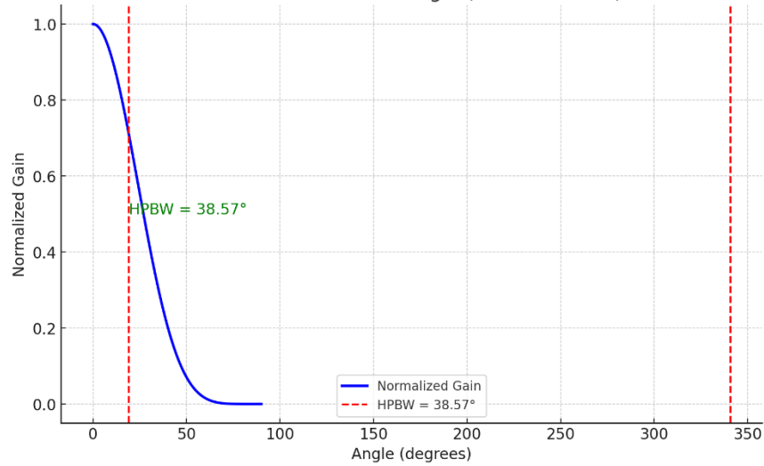
Normalized Gain vs Angle (Cartesian Plot)
