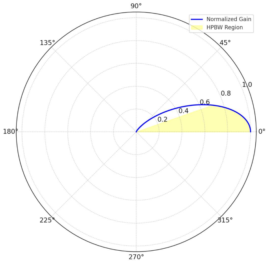
Antenna Radiation Pattern (Polar Plot)
